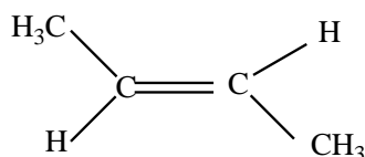
Trans isomer
