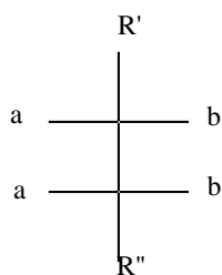
erythro form
