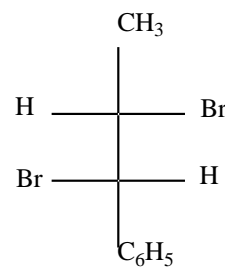
threo form
