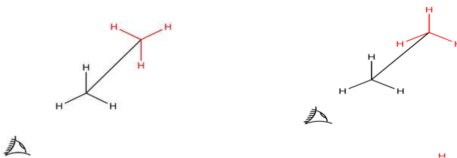
Anti conformation
