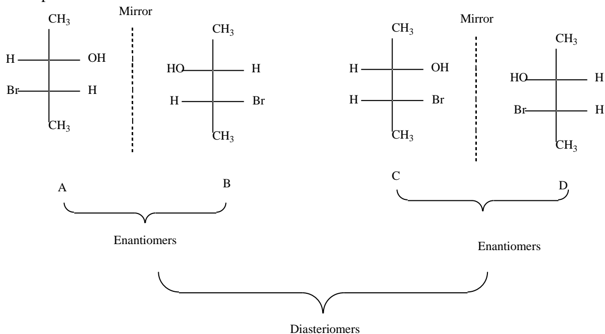
Four isomers of 3-Bromo-2-butanol
