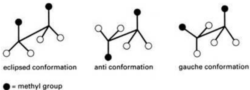
eclipsed conformation
