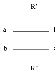
threo form
