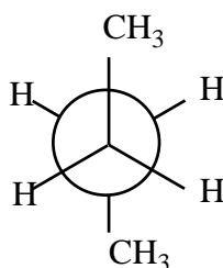
Anti
