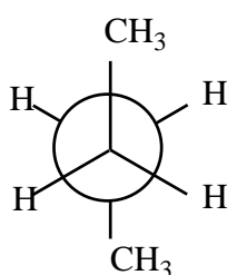
Anti
