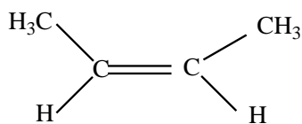
Cis isomer
