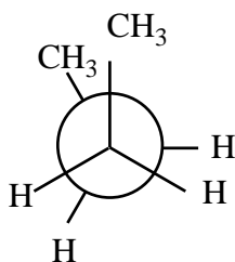
Eclipsed
