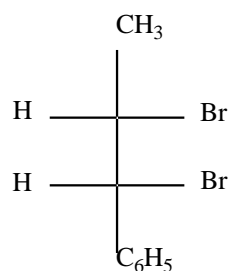
erythro form
