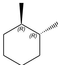
Trans isomer
