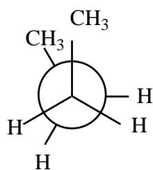
Eclipsed
