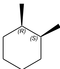
Cis isomer
